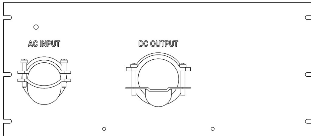
Figure 2-1 - HPX AC Input & DC Output Strain Relief Panel (Rack Output Current \leq 1000A )
