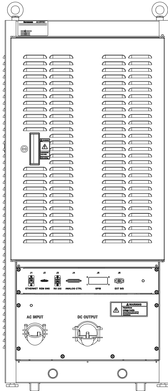
Figure 2-13 - 24U HPX Power Rack, Rear View
