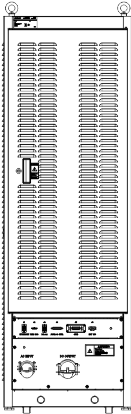
Figure 2-14 - 35U HPX Power Rack, Rear View
