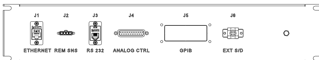
Figure 2-8 - HPX I/O Panel
