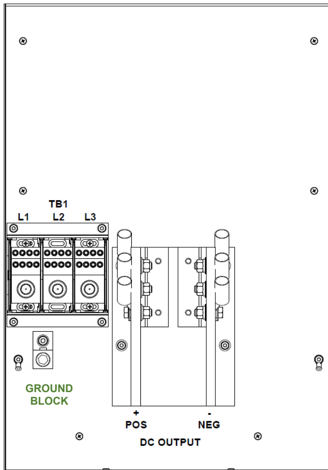
Figure 2-5 - Power Distribution Tray: “Internal” Bus Bar Output (400A - 2505A)
