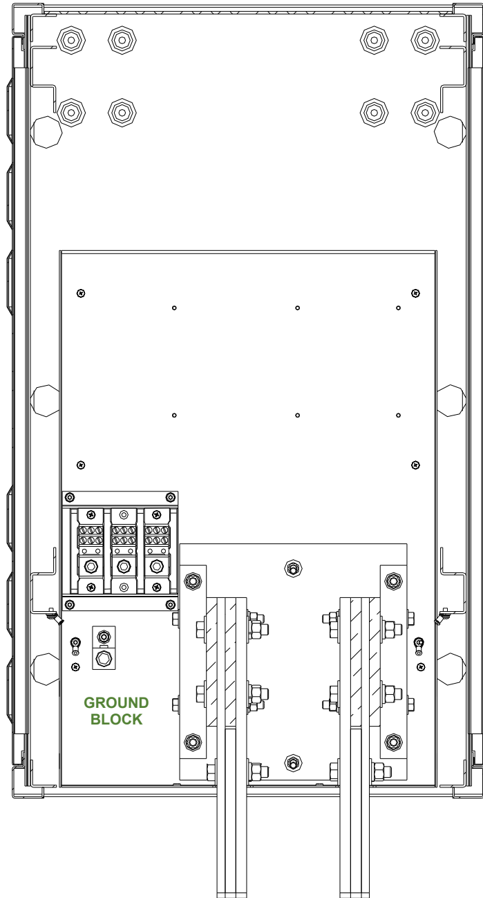
Figure 2-6 – Power Distribution Tray: Bus Bar Output (to 6000A)
