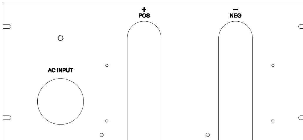
Figure 2-2 - HPX AC Input & DC Output, Bus Bar configuration (Rack Output Current > 1000A )
