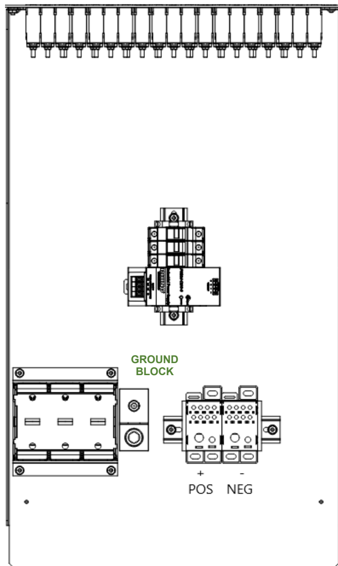
Figure 2-4 - Power Distribution Tray: Terminal block output (0-299A)
