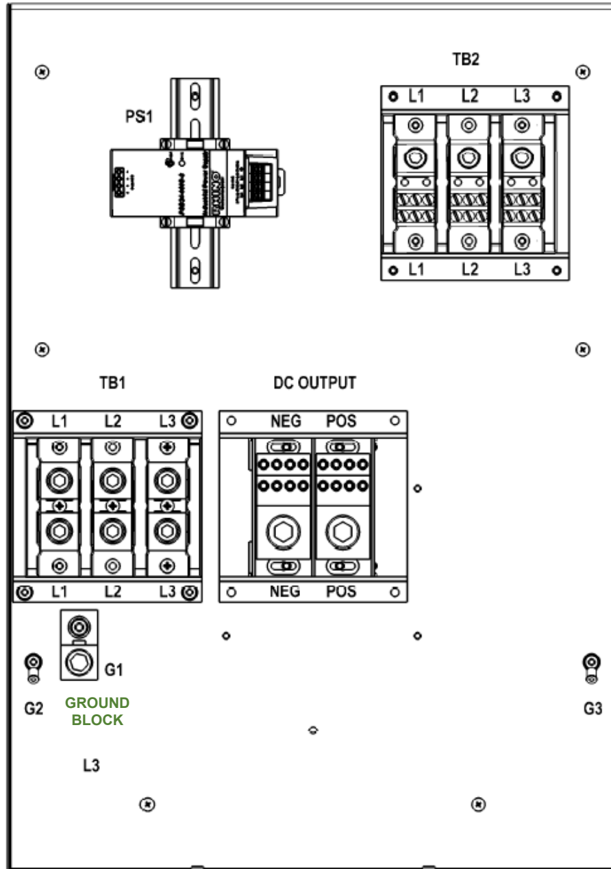
Figure 2-3 - Power Distribution Tray: AC Input & DC Output Terminal Blocks (< 400A)
