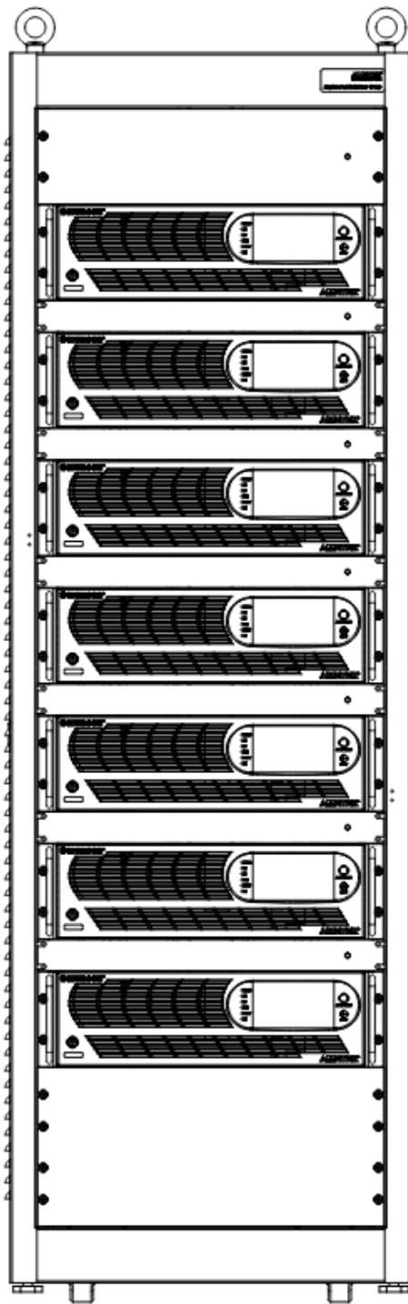
Figure 2-10 - 35U HPX Power Rack, Front View
