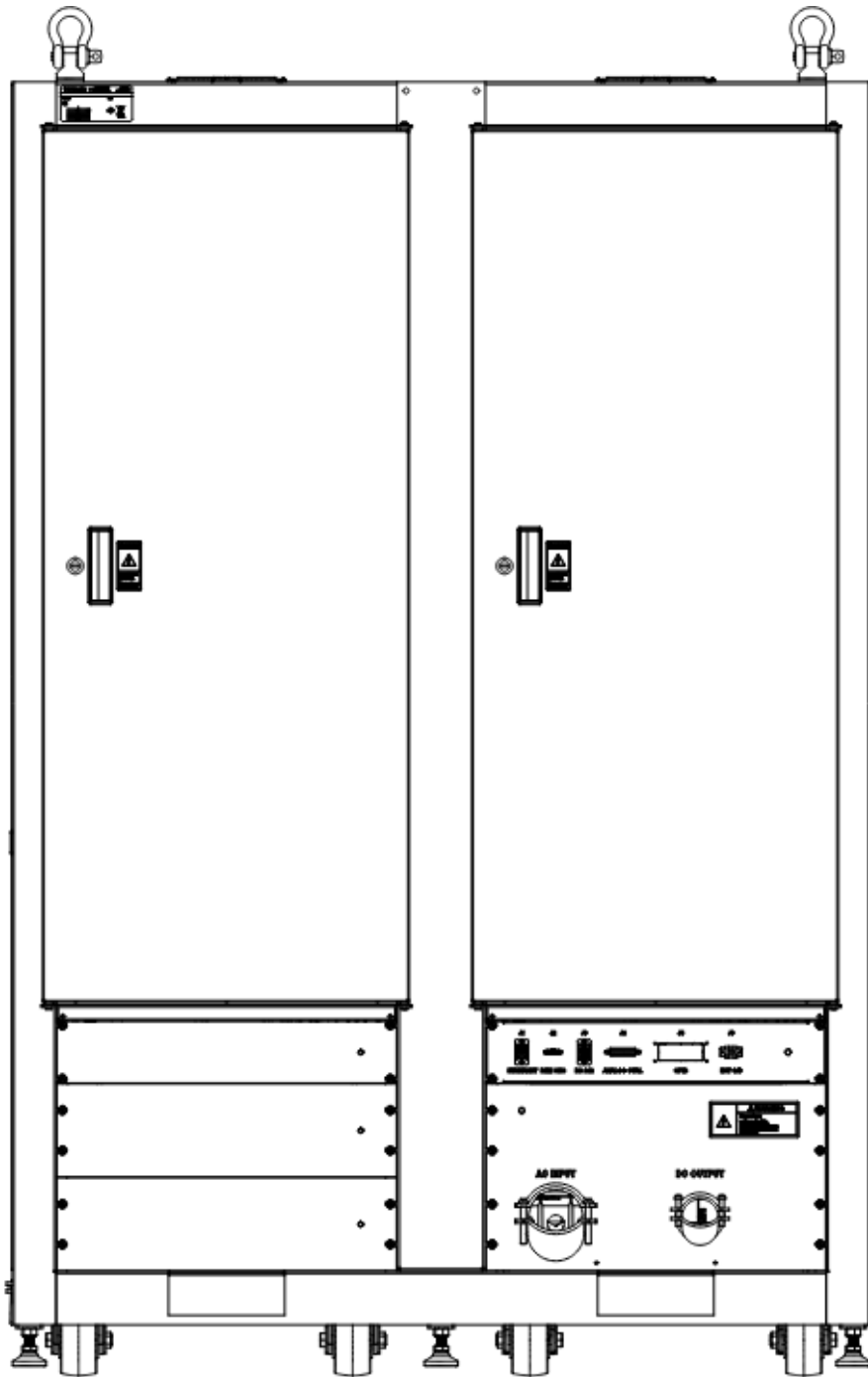
Figure 2-16 – 2x36U HPX Power Rack, Rear View
