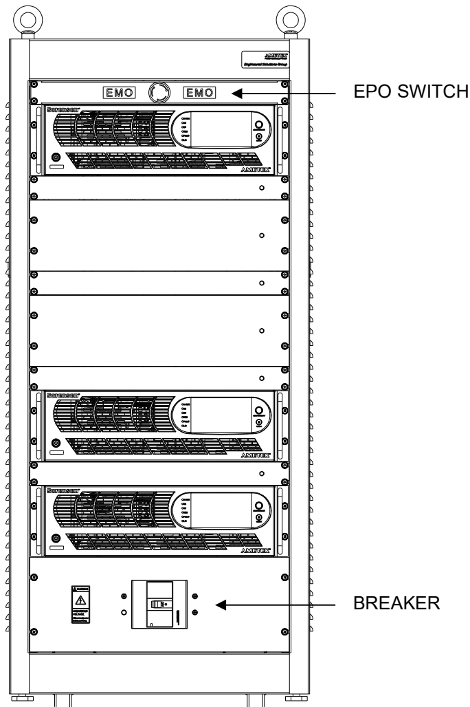
Figure 1-5 - 24U Rack w/ Circuit Breaker & EPO Switch Option
