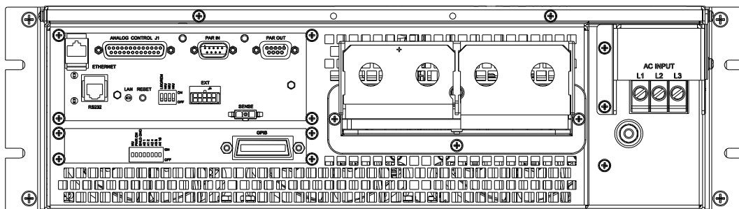
Figure 1-2 – SGX Power Supply Rear View (10-30V)
