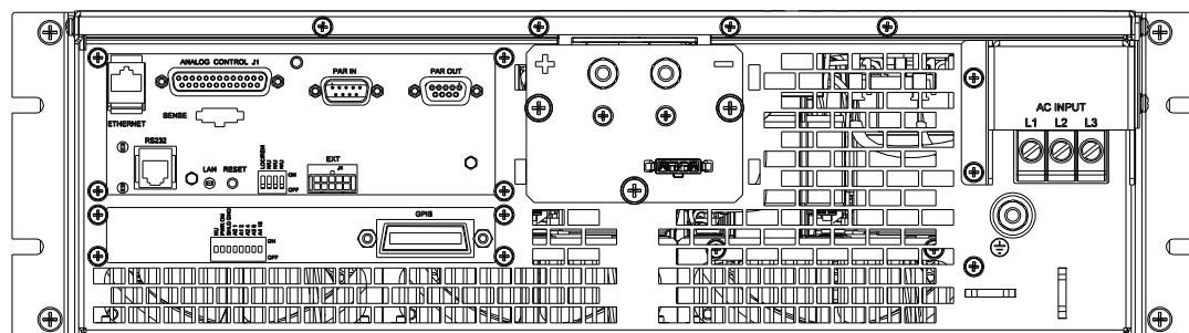
Figure 1-4 - SGX POWER SUPPLY (800/1000V)
